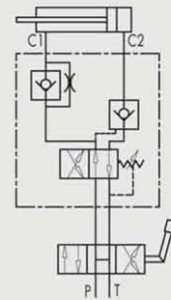
SCHEMA IDRAULICO HYDRAULIC DIAGRAM
