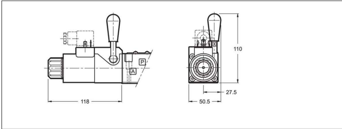
13.2 - CH-DS3/10 Lever manual override (only for DC solenoid valve)
